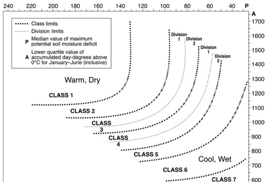
Fig. 1. The 2-parameter climate classification for LCA classes (figure from Bibby et al. 1982)
